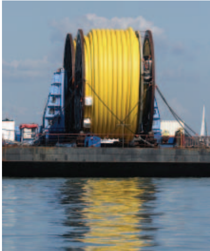
Pipe laying in the Solent
