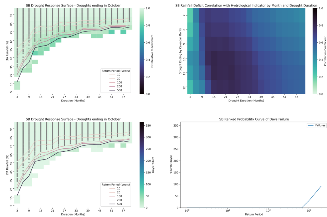
Figure 12: Drought response surface plots for SBZ.
