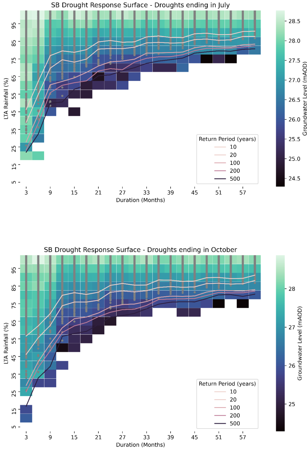
Figure 10: Drought response surface for groundwater level decline (SBZ indicator borehole).
