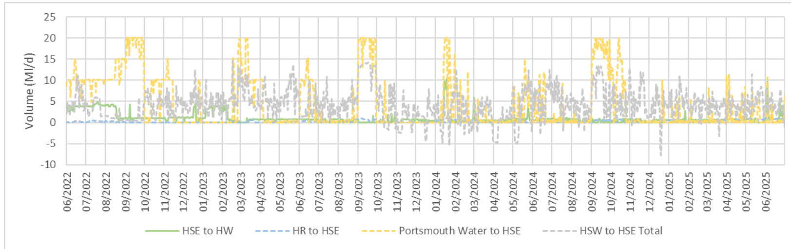
Figure 9: Daily transfers to and from HSE and bulk supply from June 2022.
