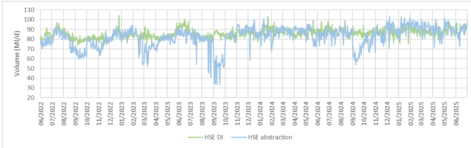
Figure 3: HSE abstraction vs. total distribution input, including transfers, from June 2022 to June 2025.
