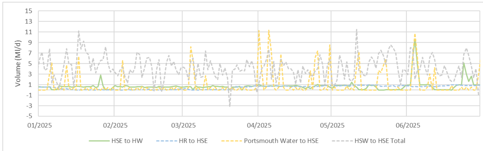
Figure 10: Daily transfers to and from HSE and bulk supply in 2025.
